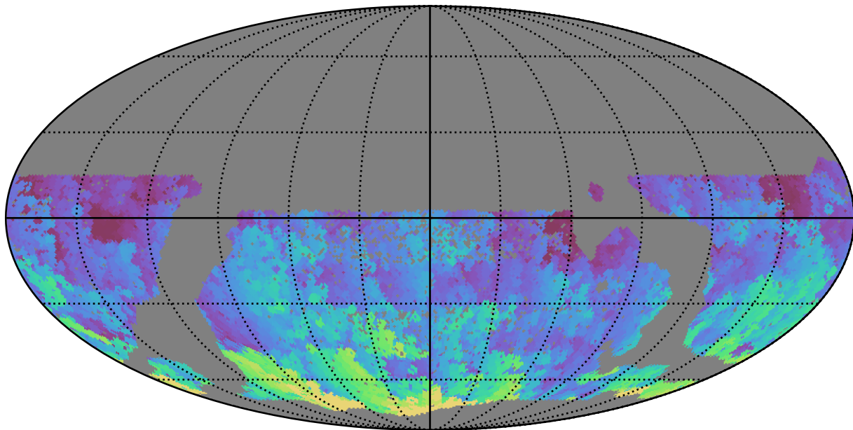
scp_reweight_v3.3_10yrs WFD g band: Max HA
