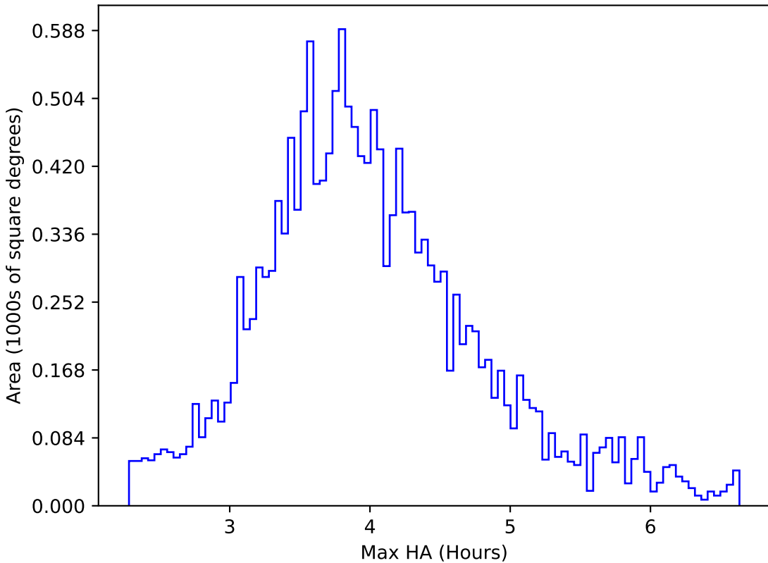
scp_reweight_v3.3_10yrs WFD g band: Max HA
