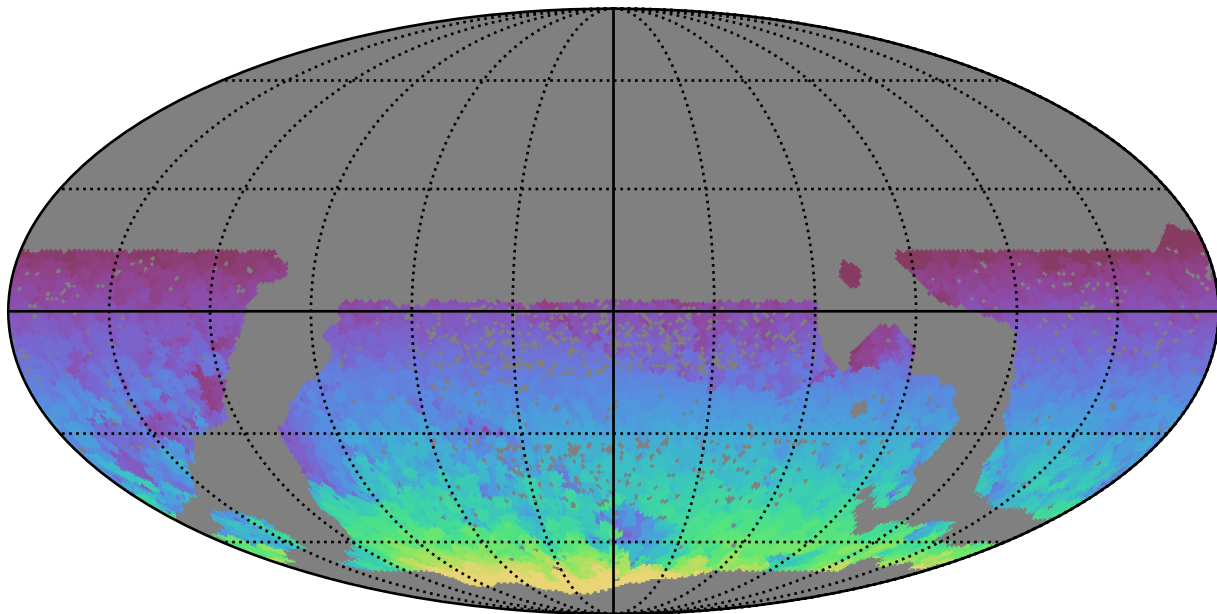
scp_reweight_v3.3_10yrs WFD all bands: Max HA
