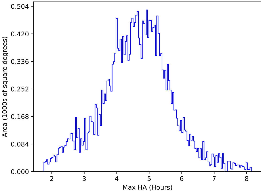
scp_reweight_v3.3_10yrs All sky z band: Max HA
