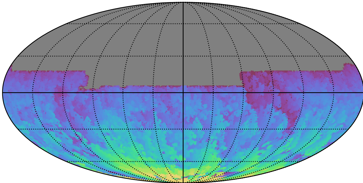
scp_reweight_v3.3_10yrs All sky y band: Max HA
