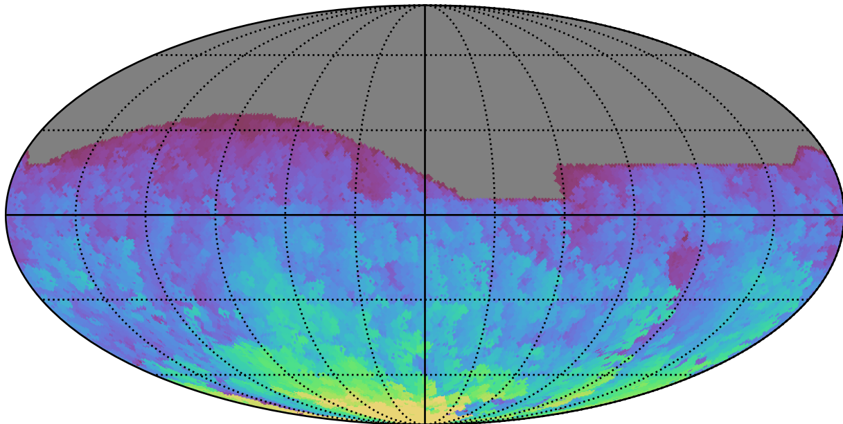
scp_reweight_v3.3_10yrs All sky r band: Max HA
