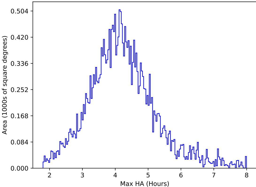
scp_reweight_v3.3_10yrs All sky r band: Max HA
