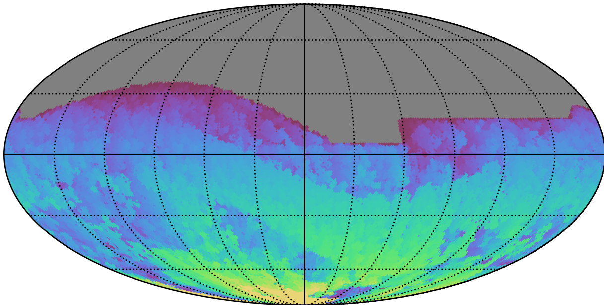
scp_reweight_v3.3_10yrs All sky i band: Max HA
