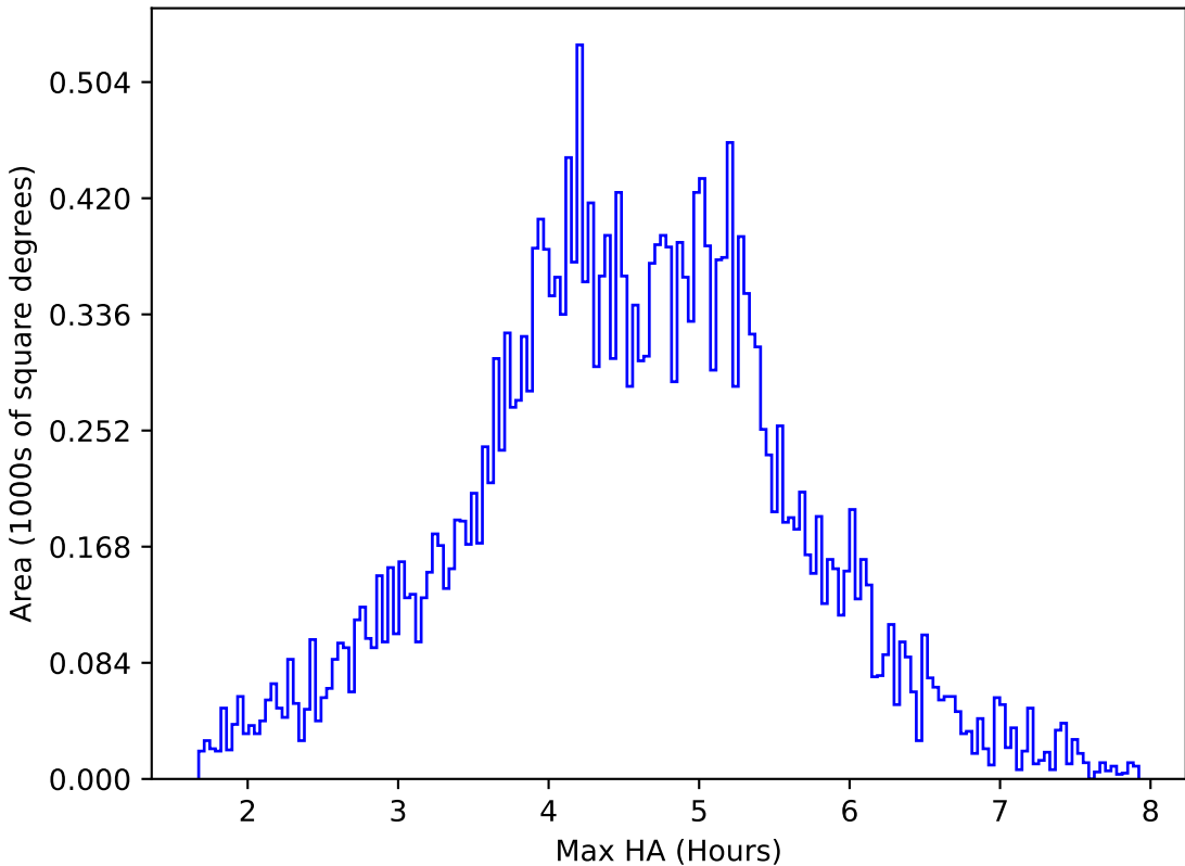
scp_reweight_v3.3_10yrs All sky i band: Max HA
