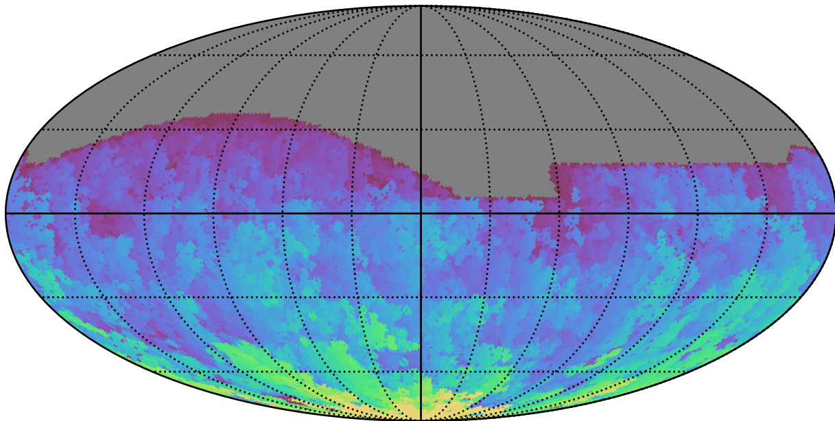
scp_reweight_v3.3_10yrs All sky g band: Max HA
