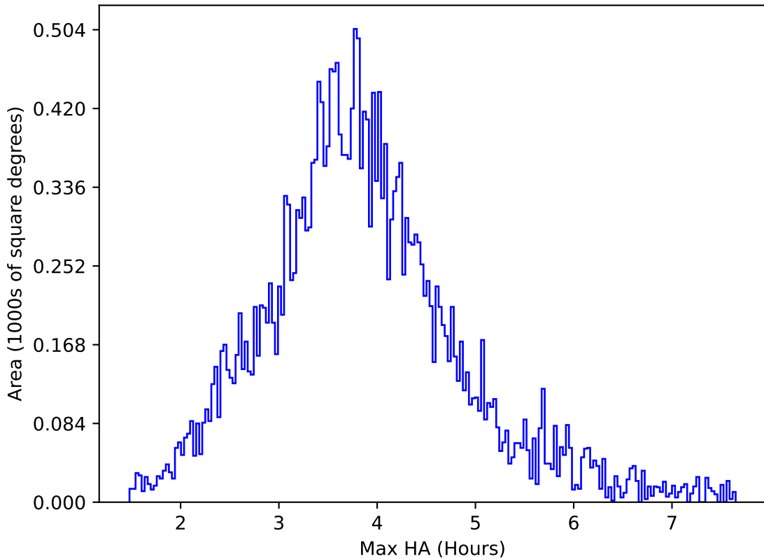
scp_reweight_v3.3_10yrs All sky g band: Max HA
