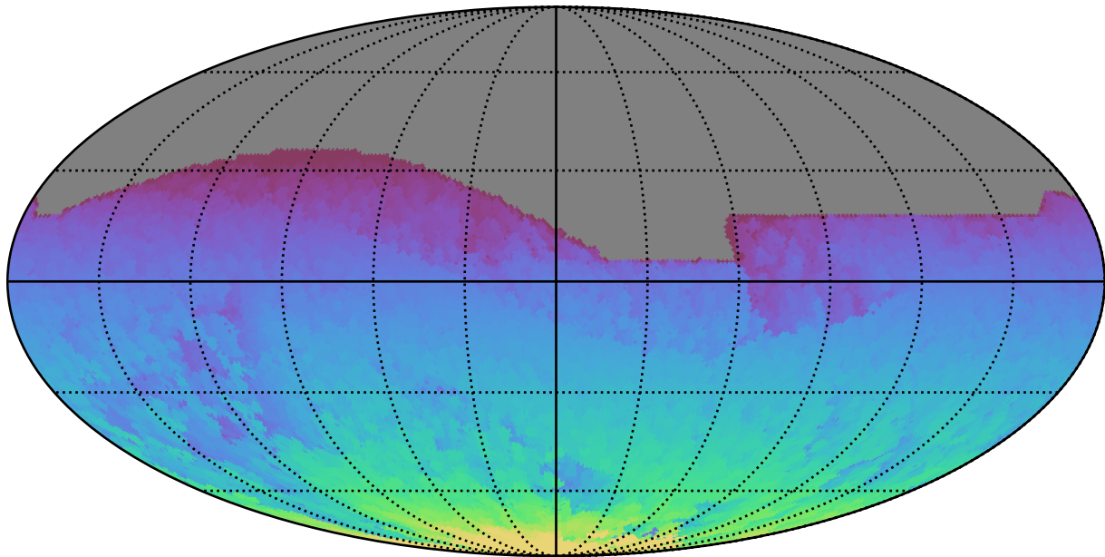
scp_reweight_v3.3_10yrs All sky all bands: Max HA
