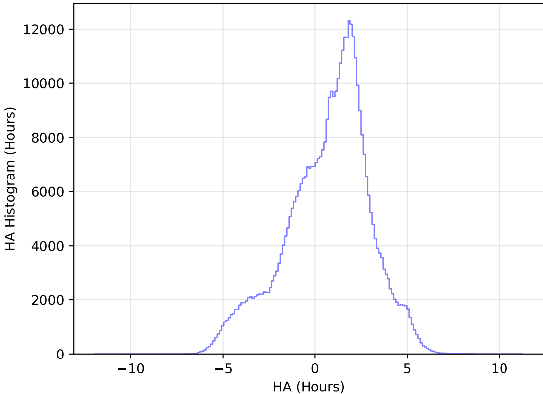
scp_reweight_v3.3_10yrs WFD z band: HA Histogram
