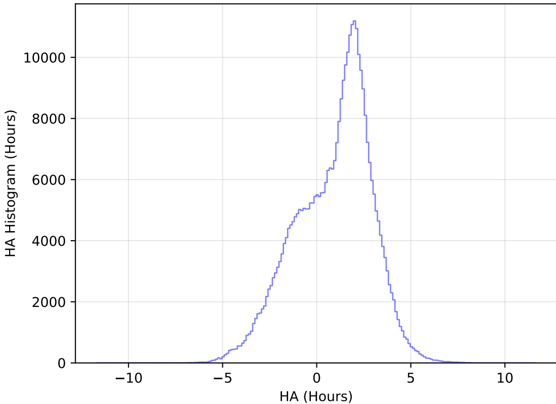
scp_reweight_v3.3_10yrs WFD y band: HA Histogram
