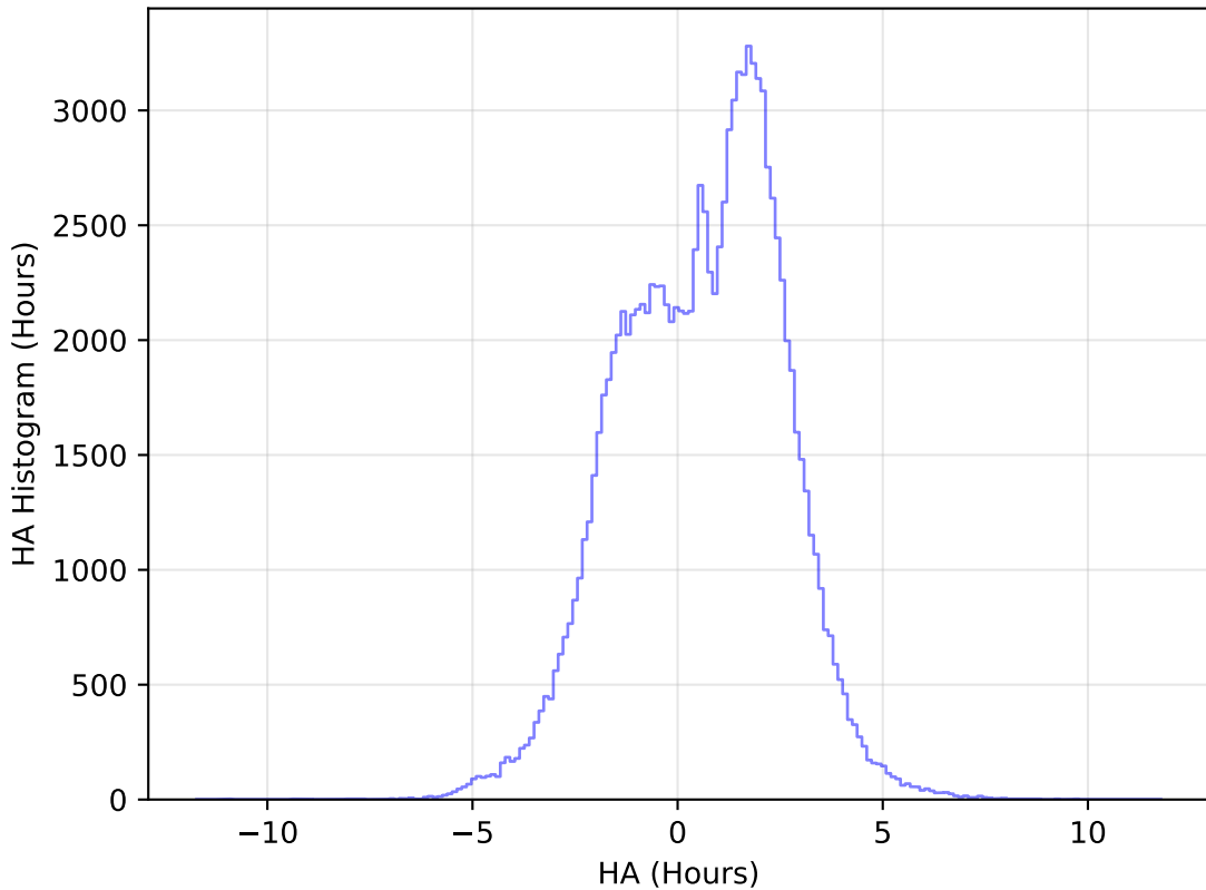
scp_reweight_v3.3_10yrs WFD u band: HA Histogram
