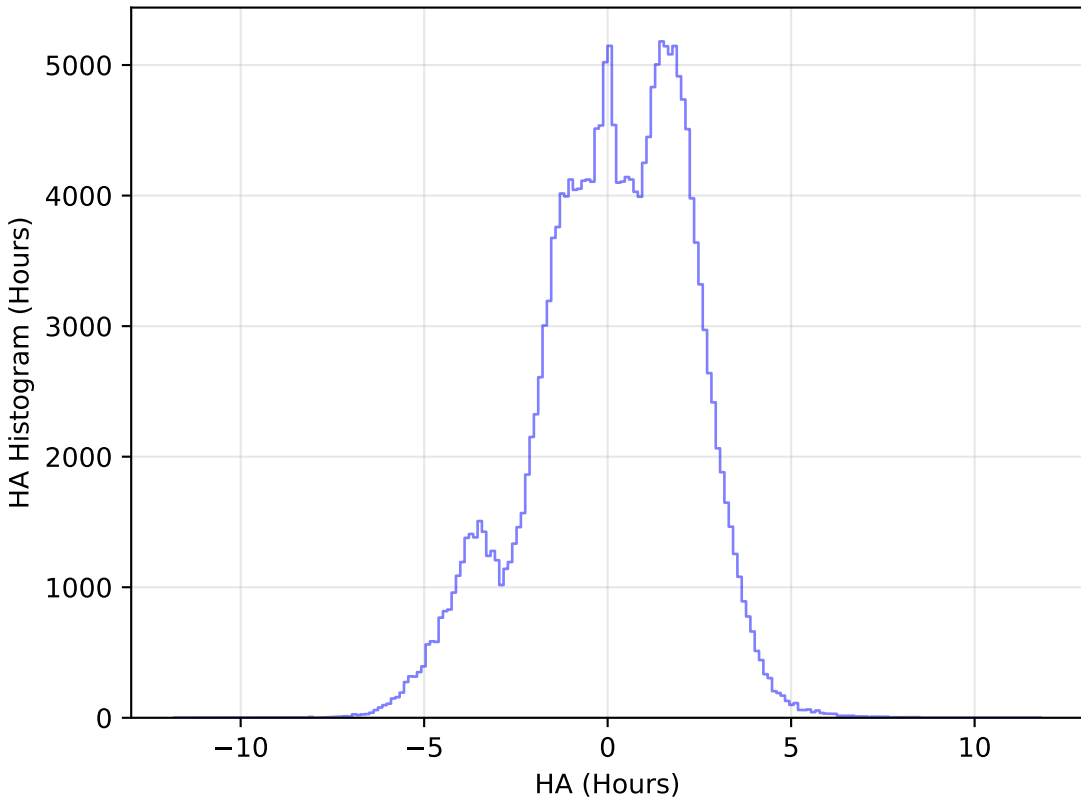
scp_reweight_v3.3_10yrs WFD g band: HA Histogram
