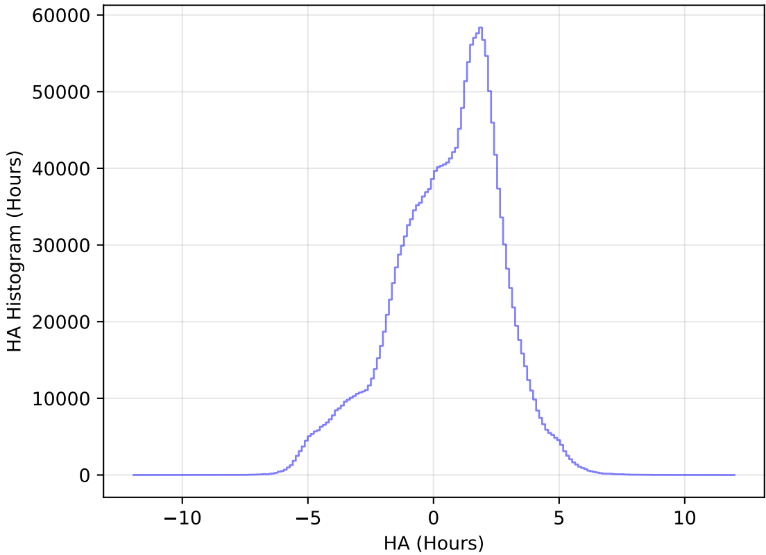
scp_reweight_v3.3_10yrs WFD all bands: HA Histogram
