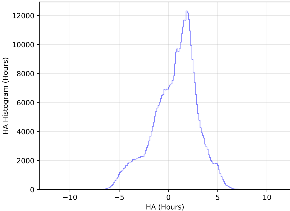
scp_reweight_v3.3_10yrs All sky z band: HA Histogram
