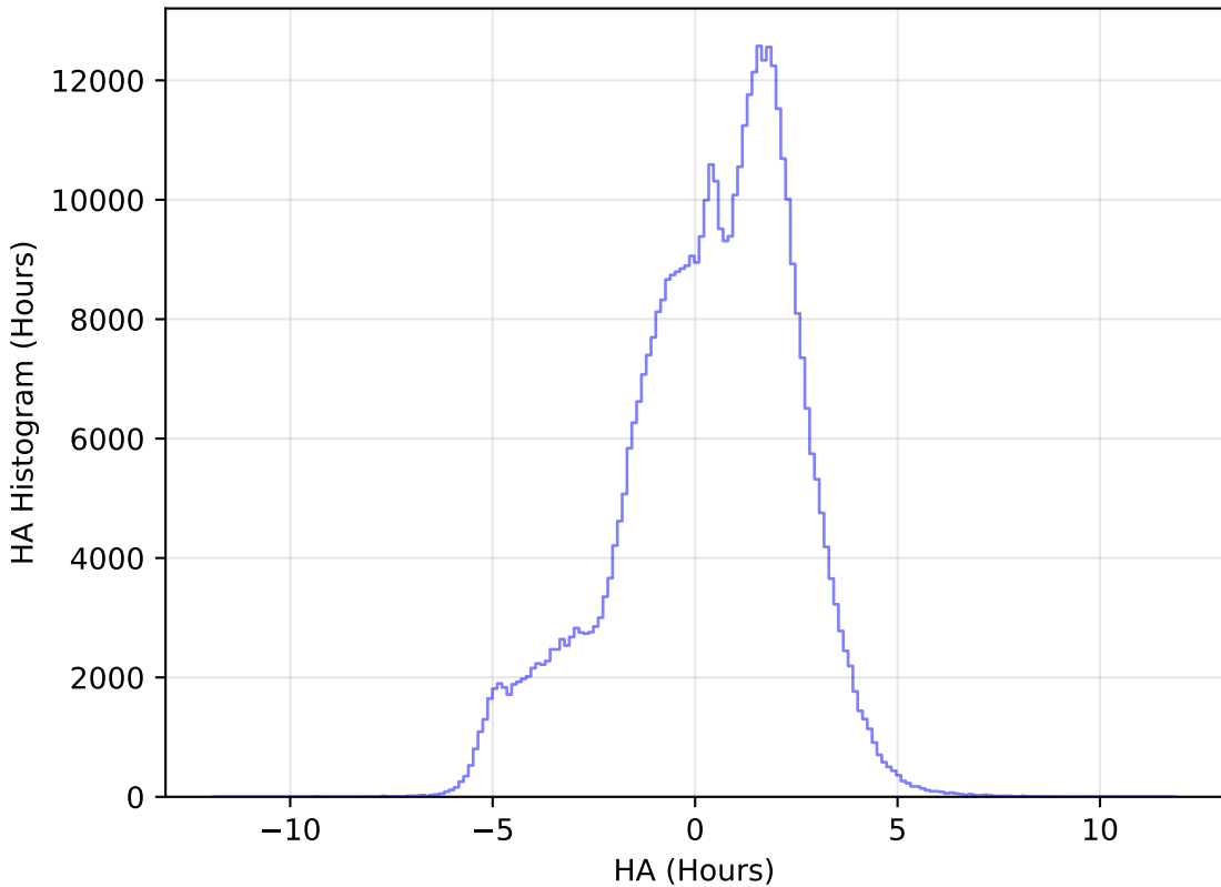
scp_reweight_v3.3_10yrs All sky r band: HA Histogram
