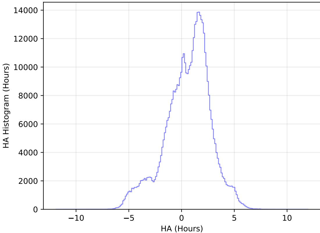
scp_reweight_v3.3_10yrs All sky i band: HA Histogram
