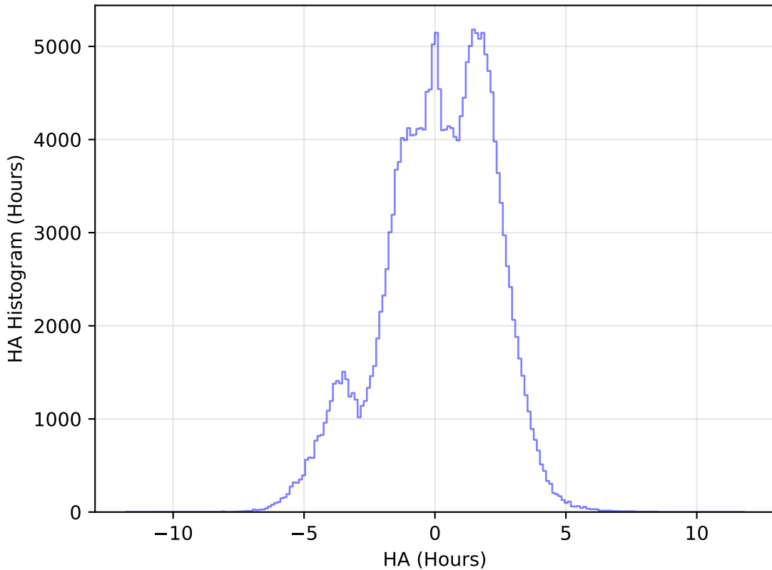
scp_reweight_v3.3_10yrs All sky g band: HA Histogram
