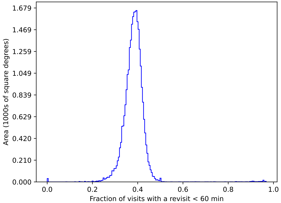
scp_reweight_v3.3_10yrs gri All sky: Fraction of visits with a revisit < 60 min
