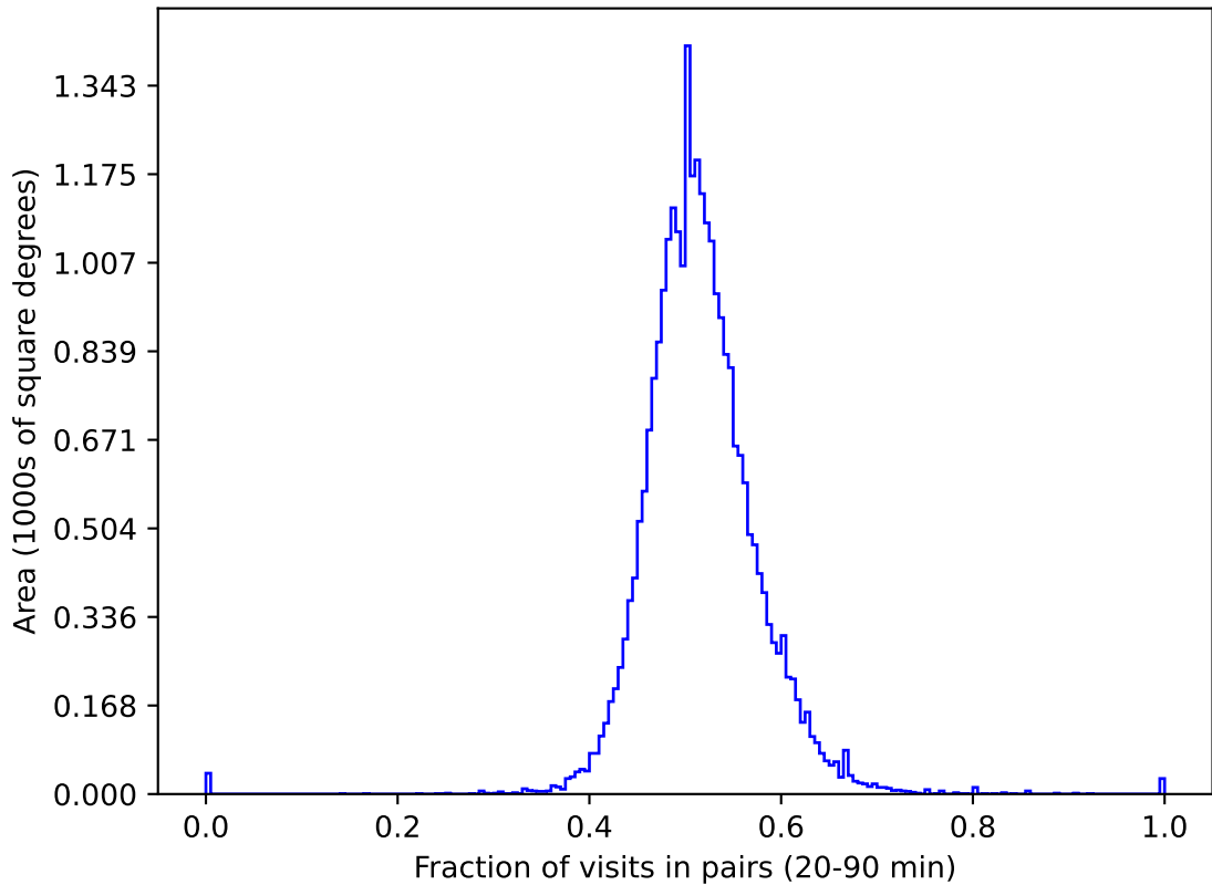
scp_reweight_v3.3_10yrs gri All sky: Fraction of visits in pairs (20-90 min)
