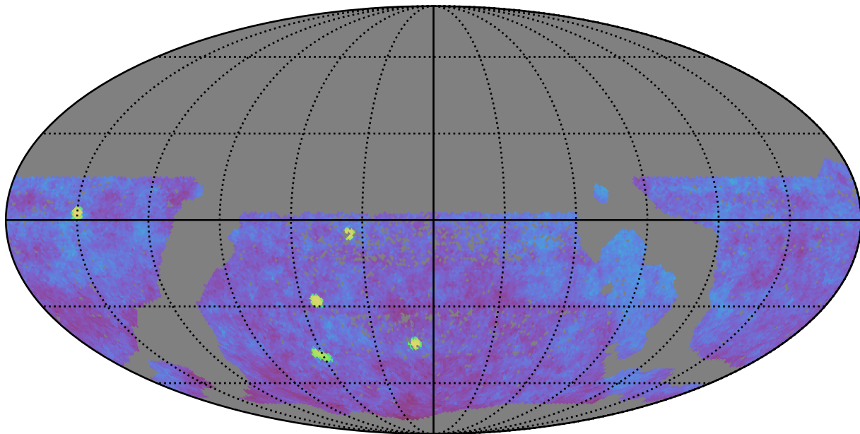
scp_reweight_v3.3_10yrs gri WFD: Fraction of visits in pairs (10-60 min)
