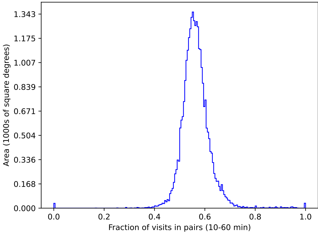
scp_reweight_v3.3_10yrs gri All sky: Fraction of visits in pairs (10-60 min)
