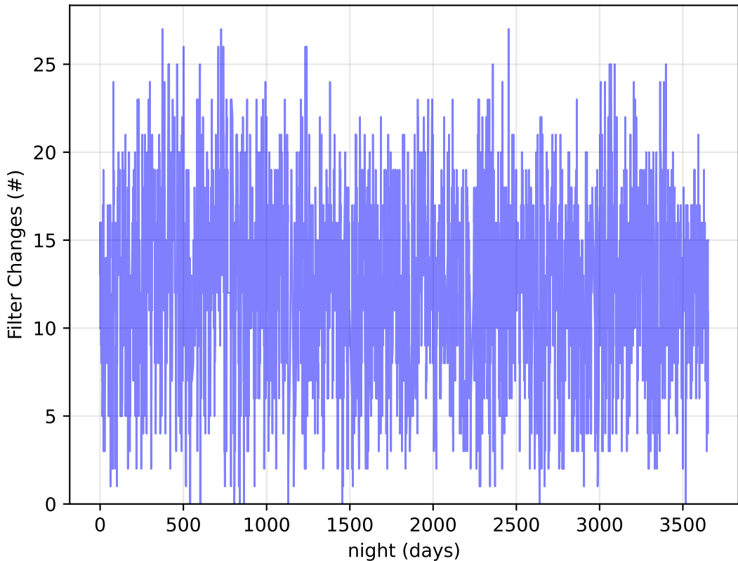
scp_reweight_v3.3_10yrs Per Night: Filter Changes
