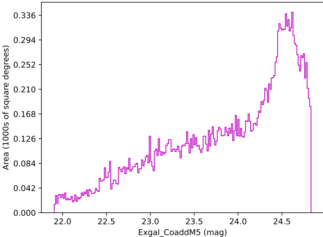
scp_reweight_v3.3_10yrs Yr 3-4 z band: Exgal_CoaddM5
