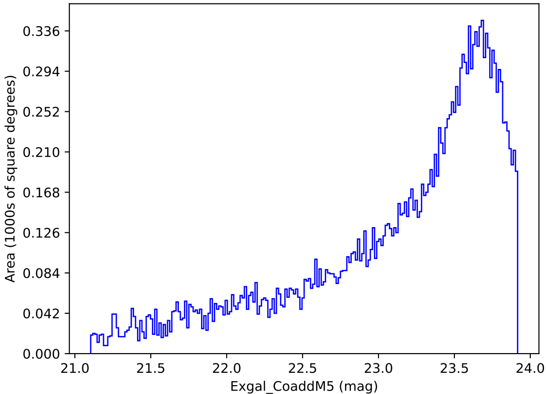
scp_reweight_v3.3_10yrs Yr 3-4 y band: Exgal_CoaddM5
