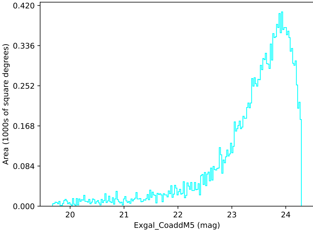
scp_reweight_v3.3_10yrs Yr 3-4 u band: Exgal_CoaddM5
