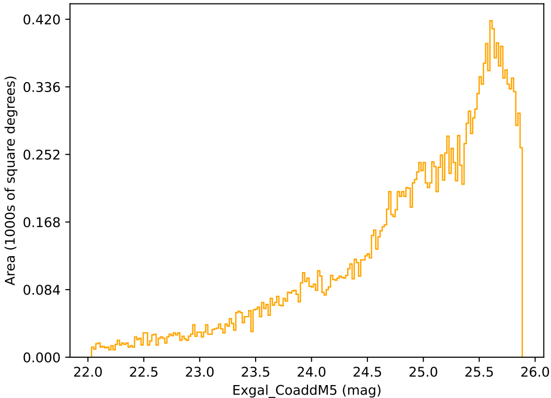
scp_reweight_v3.3_10yrs Yr 3-4 r band: Exgal_CoaddM5
