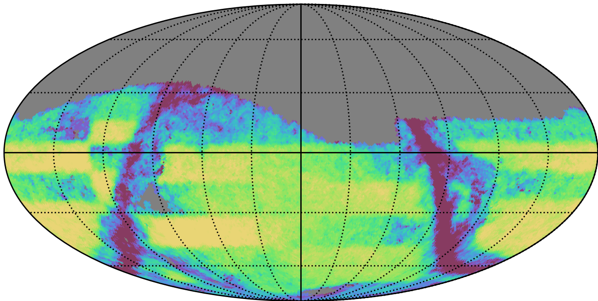
scp_reweight_v3.3_10yrs Yr 3-4 i band: Exgal_CoaddM5
