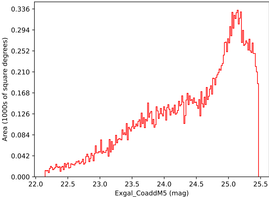
scp_reweight_v3.3_10yrs Yr 3-4 i band: Exgal_CoaddM5
