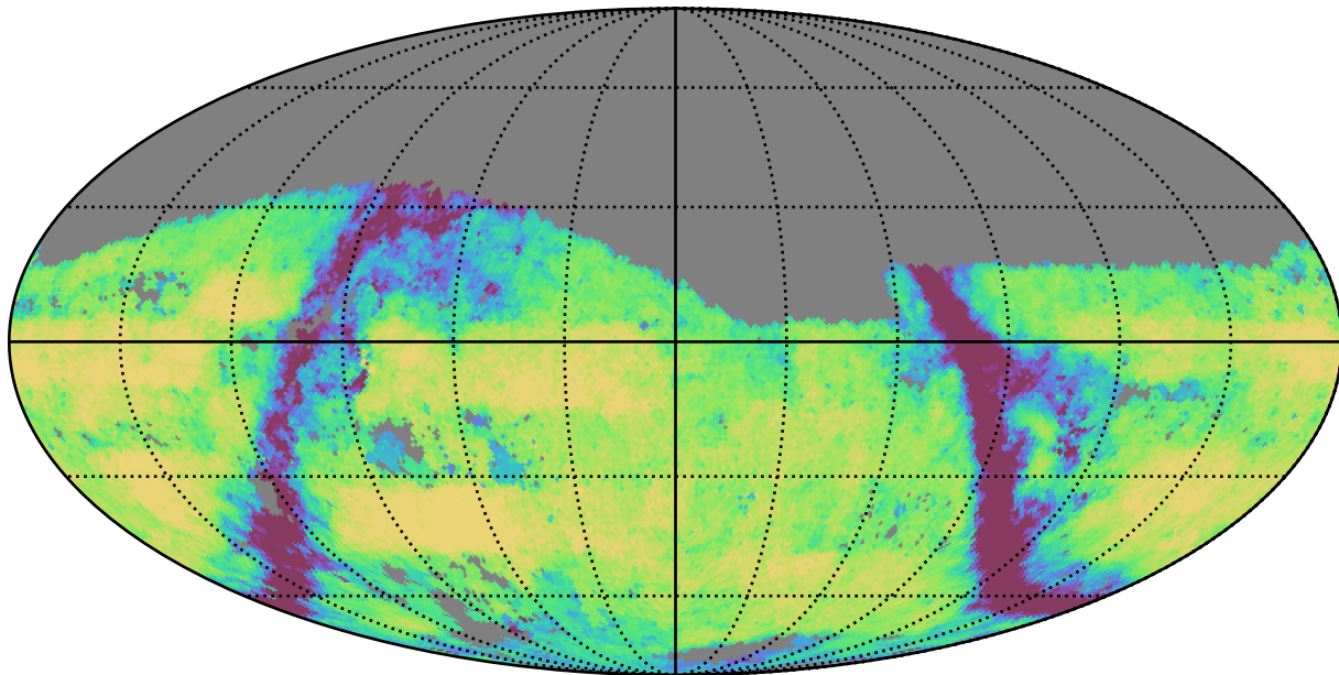
scp_reweight_v3.3_10yrs Yr 3-4 g band: Exgal_CoaddM5
