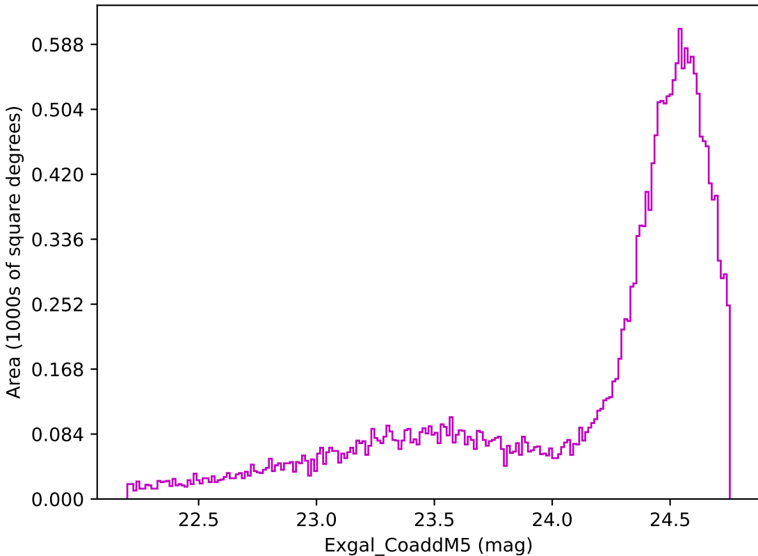
scp_reweight_v3.3_10yrs Yr 1 z band: Exgal_CoaddM5
