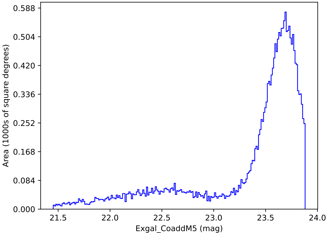
scp_reweight_v3.3_10yrs Yr 1 y band: Exgal_CoaddM5
