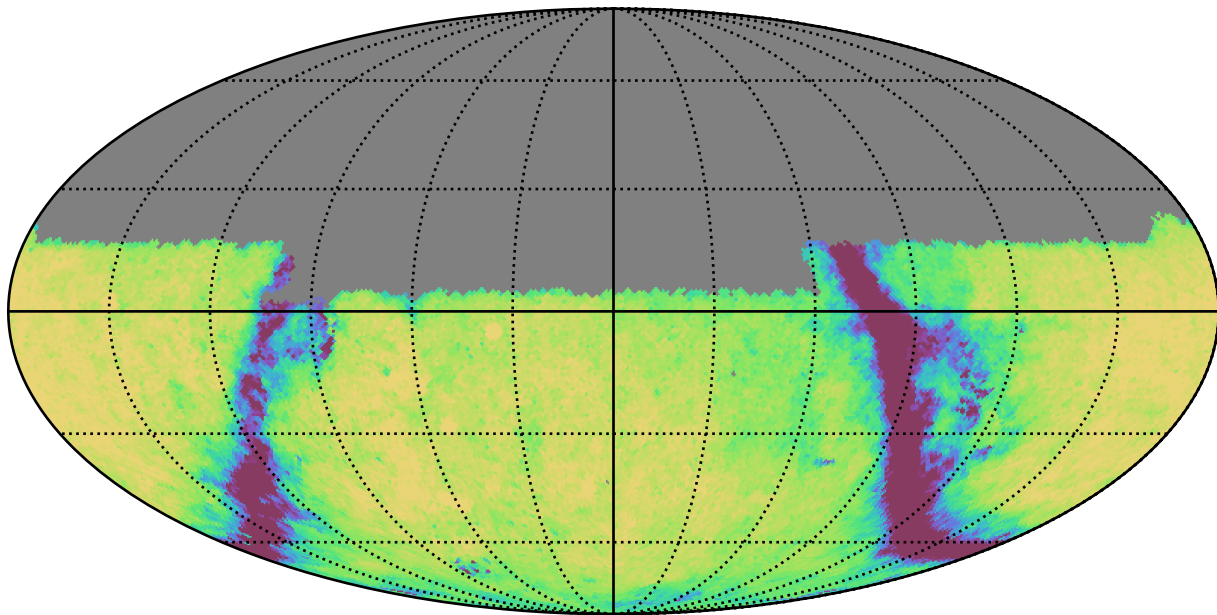
scp_reweight_v3.3_10yrs Yr 1 u band: Exgal_CoaddM5
