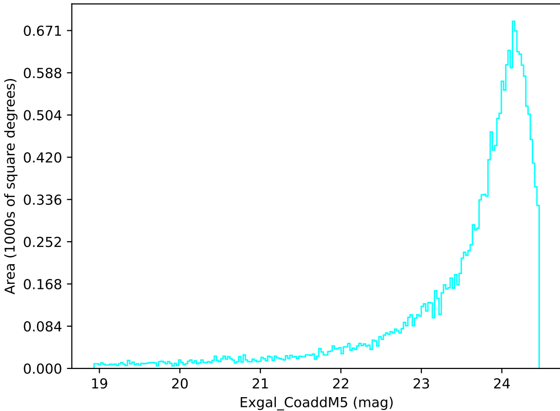
scp_reweight_v3.3_10yrs Yr 1 u band: Exgal_CoaddM5
