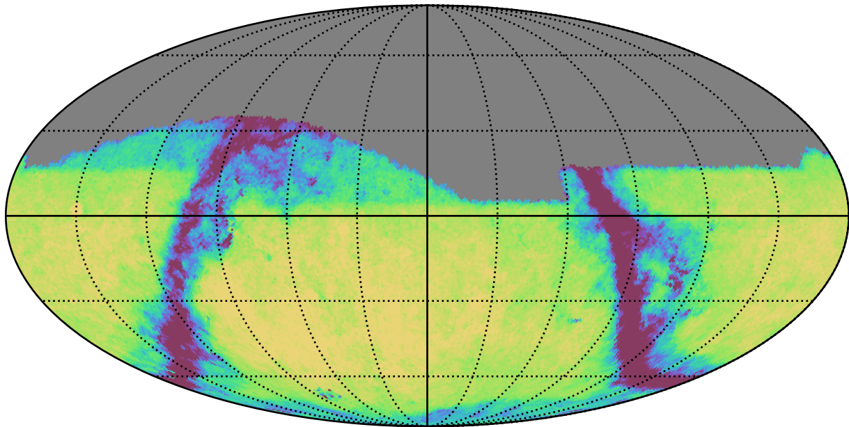
scp_reweight_v3.3_10yrs Yr 1 r band: Exgal_CoaddM5
