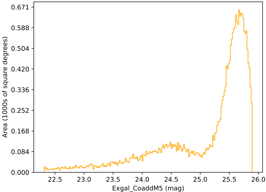
scp_reweight_v3.3_10yrs Yr 1 r band: Exgal_CoaddM5
