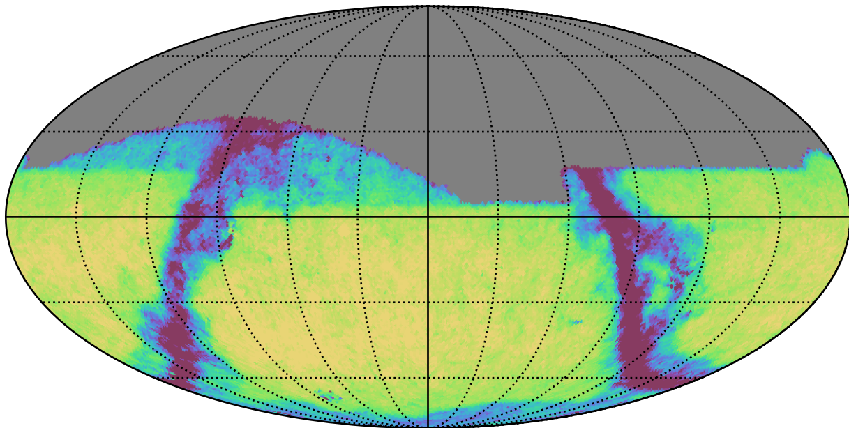
scp_reweight_v3.3_10yrs Yr 1 i band: Exgal_CoaddM5
