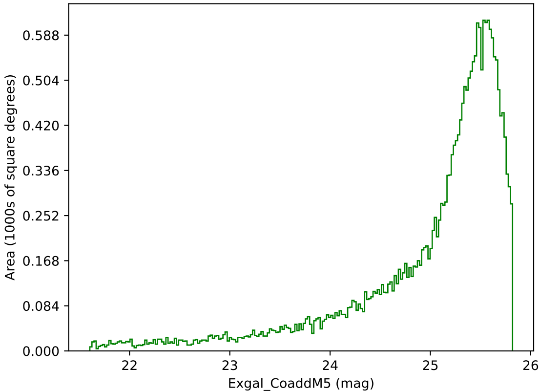
scp_reweight_v3.3_10yrs Yr 1 g band: Exgal_CoaddM5
