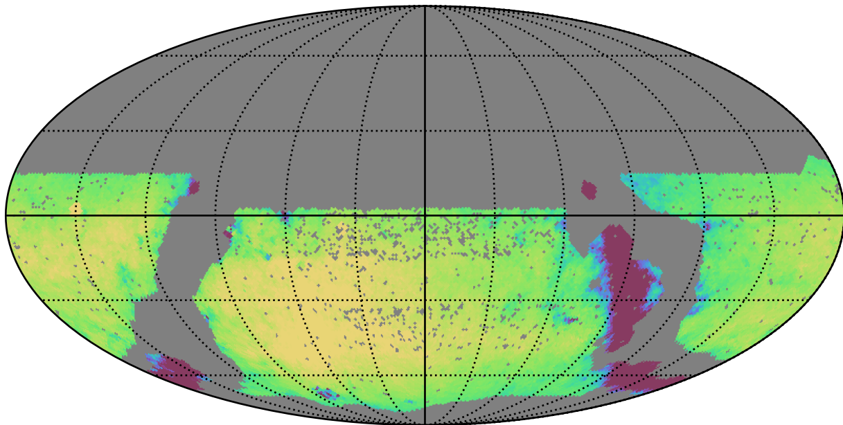
scp_reweight_v3.3_10yrs WFD r band: Exgal_CoaddM5
