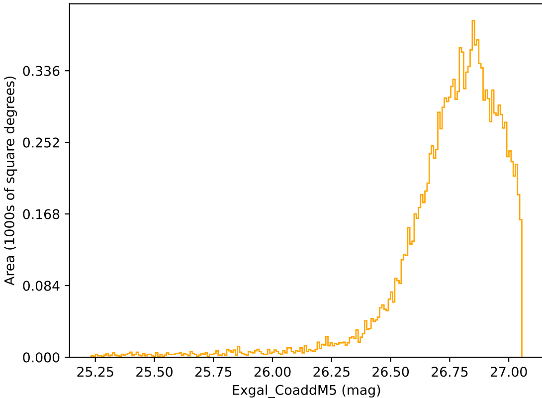
scp_reweight_v3.3_10yrs WFD r band: Exgal_CoaddM5
