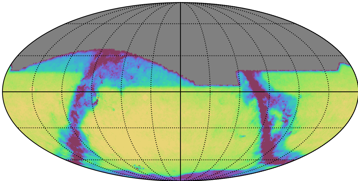
scp_reweight_v3.3_10yrs All sky z band: Exgal_CoaddM5
