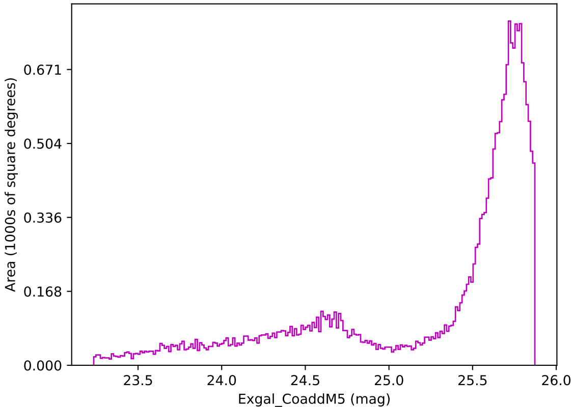
scp_reweight_v3.3_10yrs All sky z band: Exgal_CoaddM5
