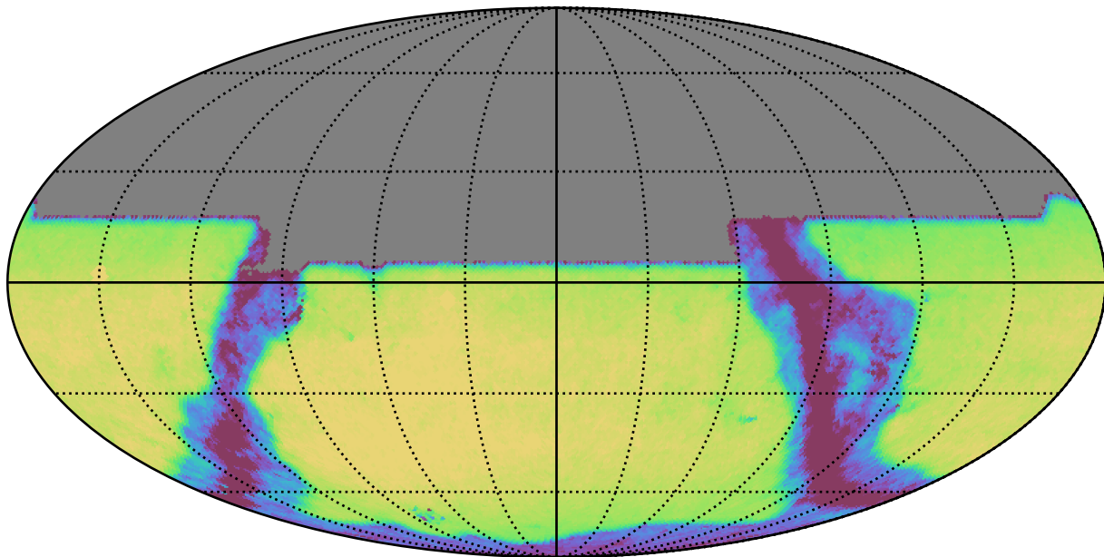
scp_reweight_v3.3_10yrs All sky y band: Exgal_CoaddM5
