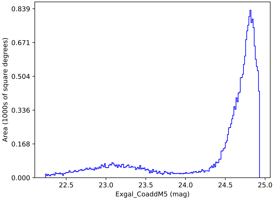
scp_reweight_v3.3_10yrs All sky y band: Exgal_CoaddM5
