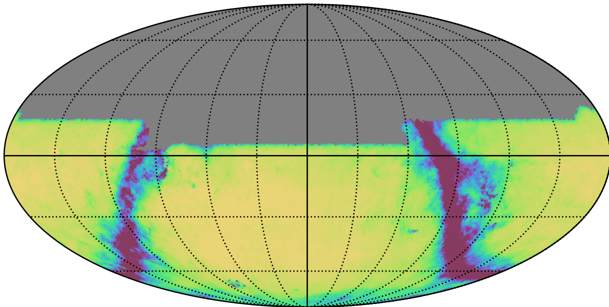
scp_reweight_v3.3_10yrs All sky u band: Exgal_CoaddM5
