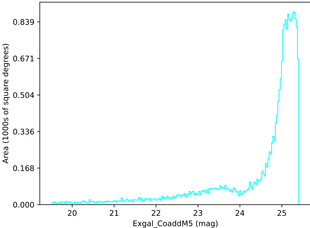
scp_reweight_v3.3_10yrs All sky u band: Exgal_CoaddM5
