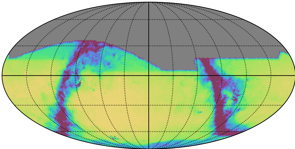
scp_reweight_v3.3_10yrs All sky r band: Exgal_CoaddM5
